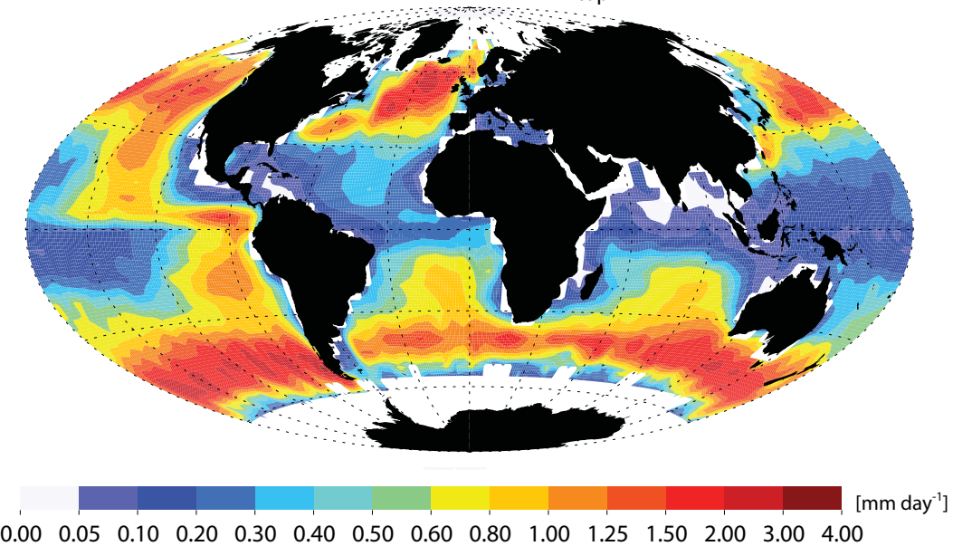
2C precipitation rate ( z_{\text{top}} < 3 \text{ km} )
