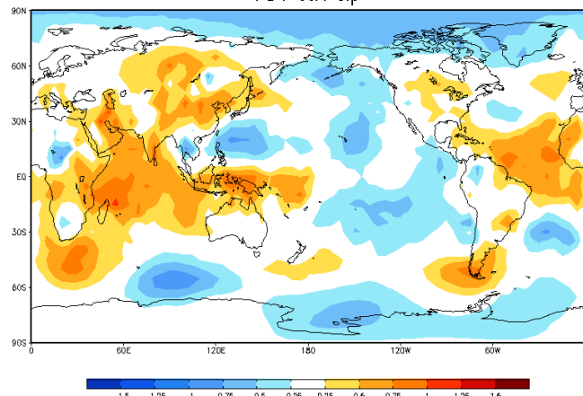
PDV JJA slp
