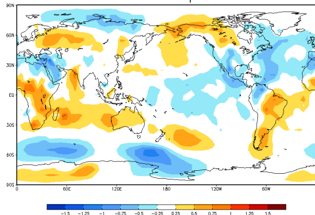
AMV JJA slp
